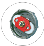
Planetary gear (L16)
